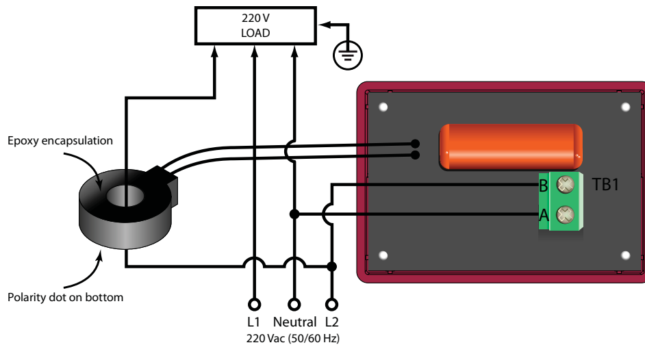
Figure 4. Wiring diagram for 220/240V systems with neutral (monitoring L2)
