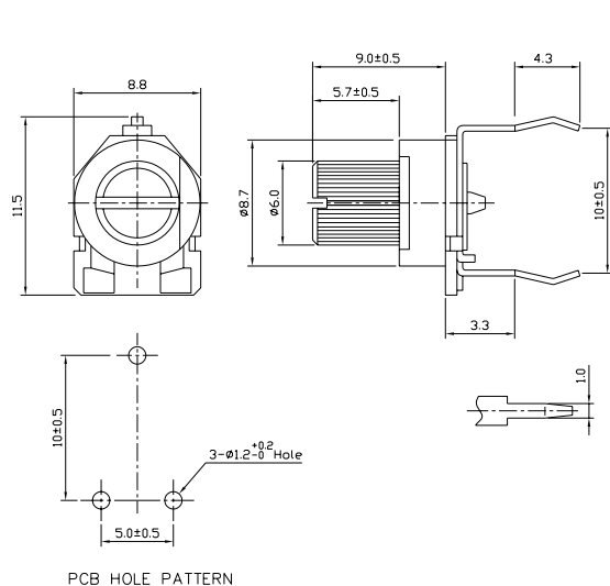
Model 37F (Top Adjust with extension)
