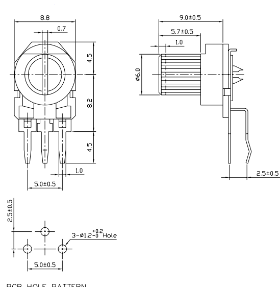
Model 37S (Side Adjust with extension)
