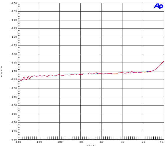
Figure 83. THD+N vs. Input Amplitude – 1 kHz Tone, 44.1 kHz:48 kHz
