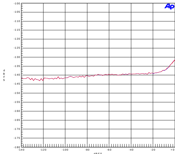
Figure 79. THD+N vs. Input Amplitude – 1 kHz Tone, 48 kHz:44.1 kHz
