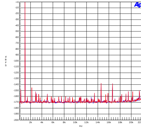
Figure 40. Wideband FFT – 0 dBFS 1 kHz Tone, 48 kHz:44.1 kHz
