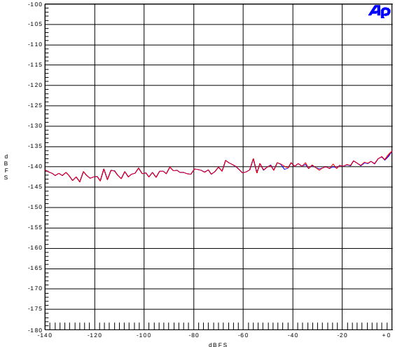
Figure 81. THD+N vs. Input Amplitude – 1 kHz Tone, 96 kHz:48 kHz
