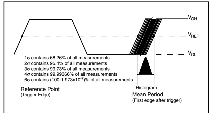
Period Jitter
