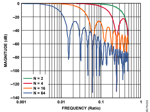
Figure 14. Bartlett Window, FIR Filter Frequency Response (Phase Delay = N Samples)
