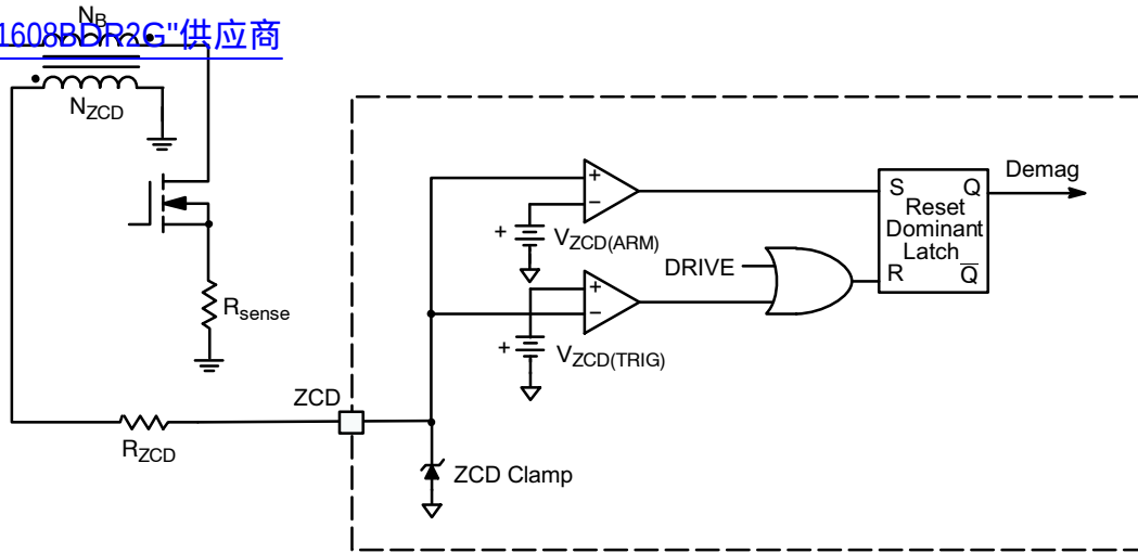
Figure 33. Implementation of the ZCD Block
