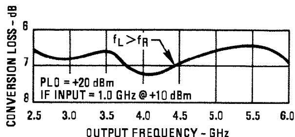
Conversion Loss (Upconversion)
