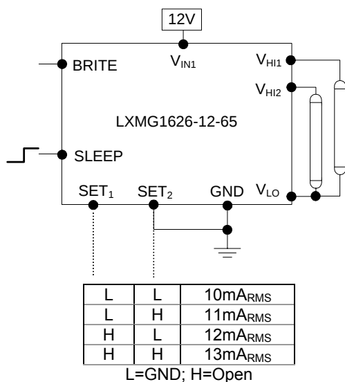
Figure 2 – Max Output Current (SET 1 and SET 2 Inputs)
