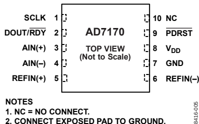
Figure 5. Pin Configuration
