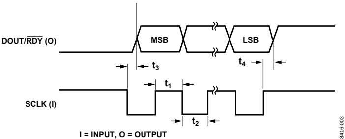
Figure 3. Read Cycle Timing Diagram
