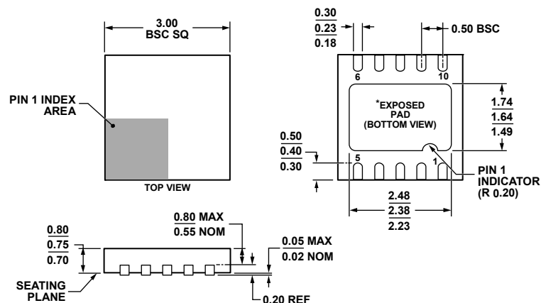
Figure 15. 10-Lead Lead Frame Chip Scale Package [LFCSP_WD] 3 mm × 3 mm Body, Very Very Thin, Dual Lead (CP-10-9) Dimensions shown in millimeters
