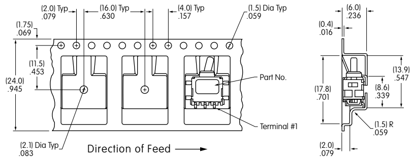
Tape Dimensions
