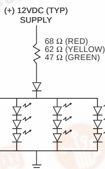
SCHEMATIC A (12V)
