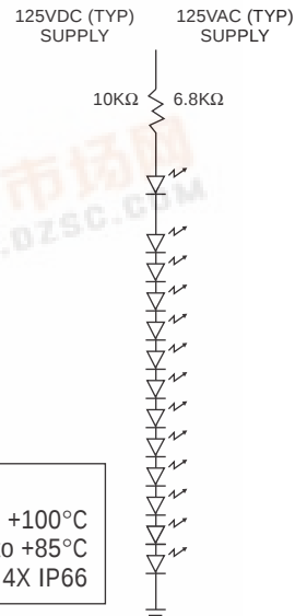
SCHEMATIC C (125V)
