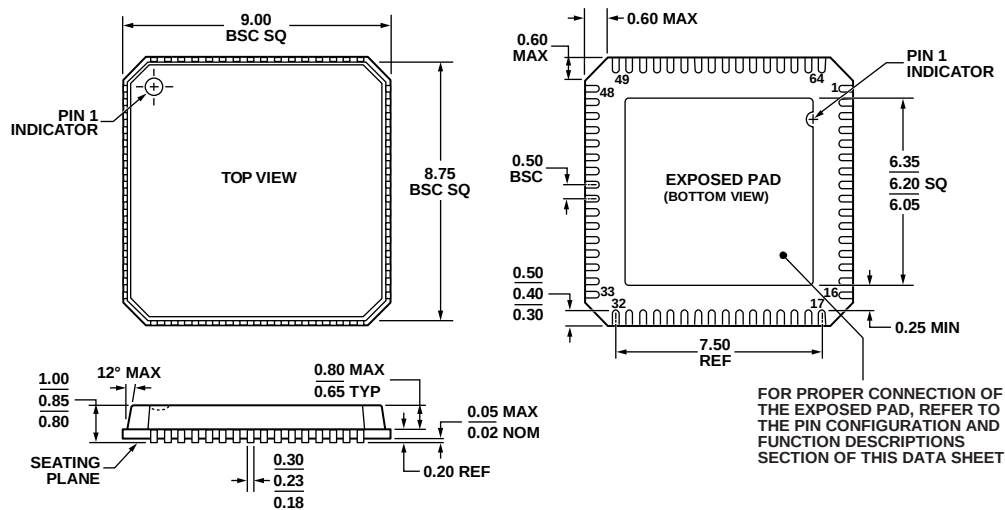
COMPLIANT TO JEDEC STANDARDS MO-220-VMMD-4 Figure 66. 64-Lead Lead Frame Chip Scale Package [LF CSP_VQ] 9 mm × 9 mm Body, Very Thin Quad (CP-64-4) Dimensions shown in millimeters
