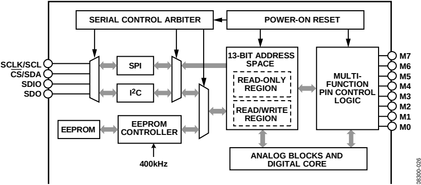
Figure 49. Serial Port Functional Diagram
