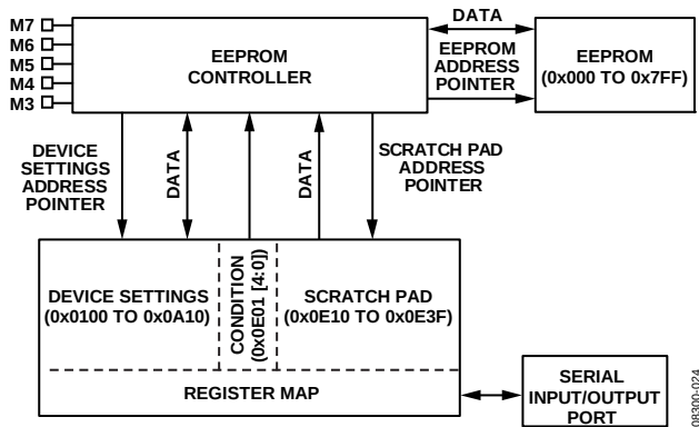
Figure 47. EEPROM Functional Diagram
