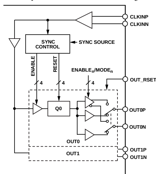
Figure 45. Clock Distribution
