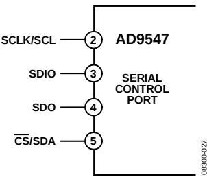
Figure 50. Serial Control Port
