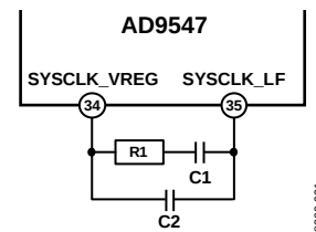
Figure 44. External Loop Filter Schematic
