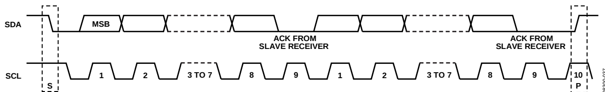
Figure 59. Acknowledge Bit
