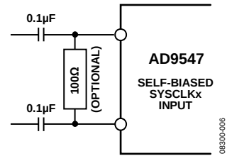
Figure 29. SYSCLKx Input
