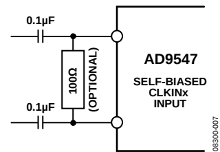
Figure 30. CLKINx Input
