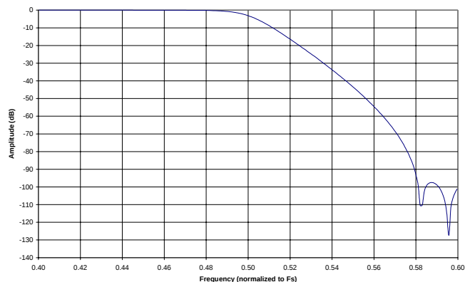
Figure 35. Single-Speed Mode Transition Band
