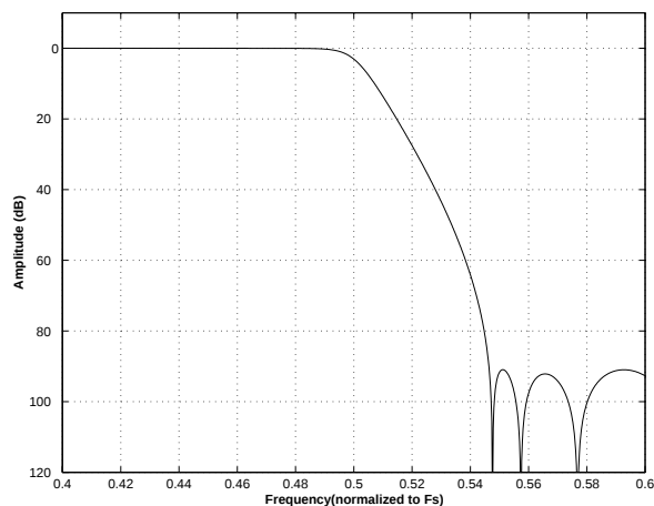
Figure 47. Single-Speed (fast) Transition Band
