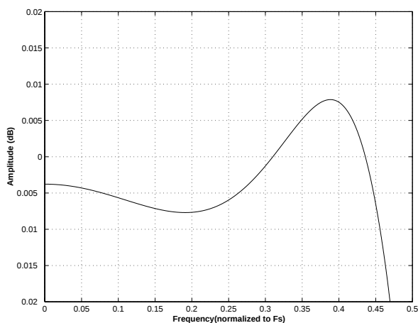
Figure 49. Single-Speed (fast) Passband Ripple
