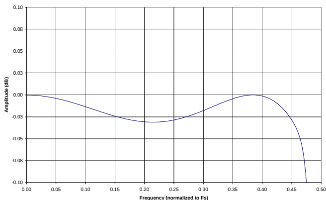
Figure 37. Single-Speed Mode Passband Ripple
