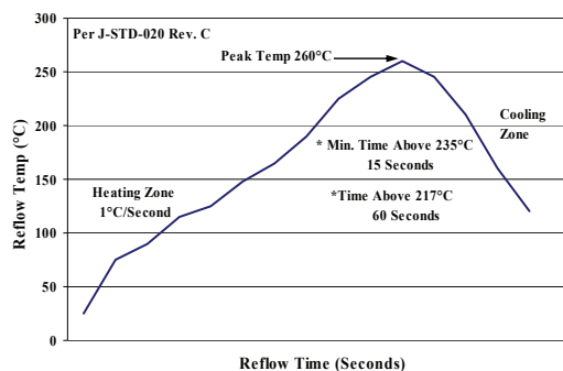
Figure 37. Recommended linear reflow profile using Sn/Ag/Cu solder.
