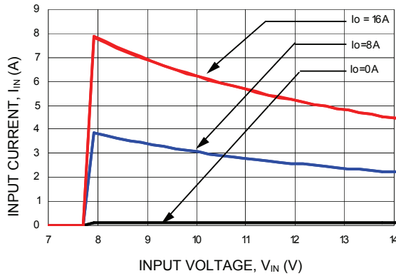
Figure 7. Input Voltage vs. Input Current ( V_O = 3.3\text{Vdc} ).
