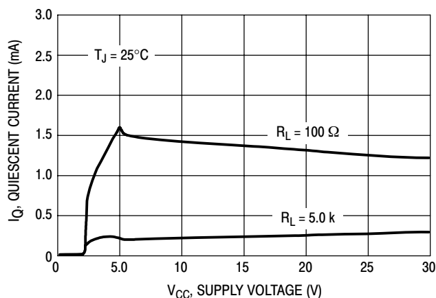
Figure 15. Quiescent Current versus Supply Voltage
