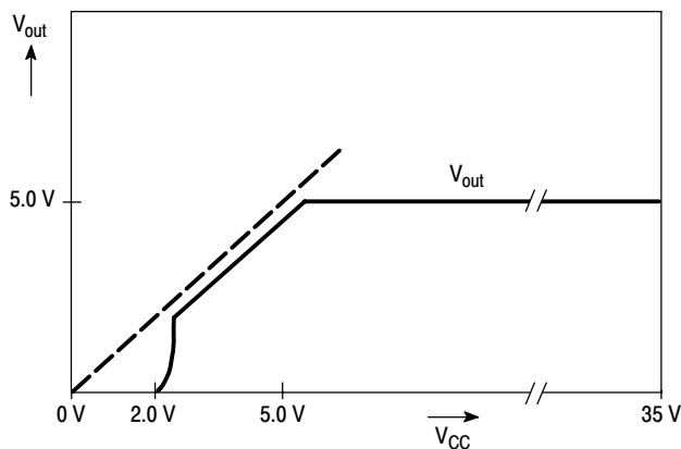
Figure 14. Output Voltage versus Supply Voltage
