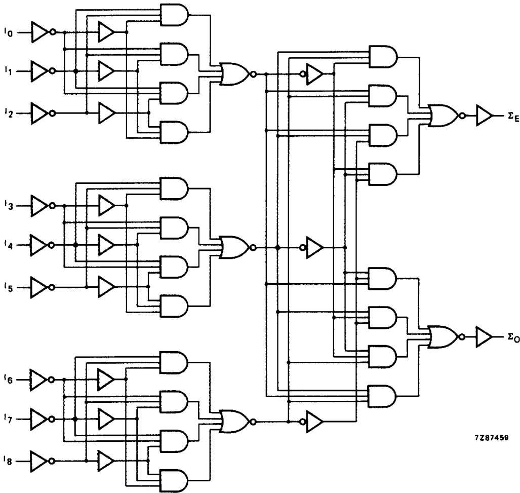
Fig.5 Logic diagram.
