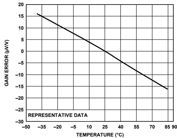
Figure 11. Gain Error vs. Temperature, Normalized at 25 ^\circ\text{C}
