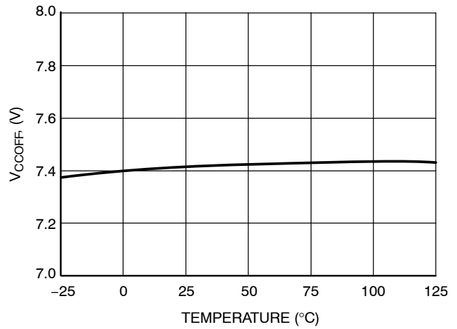
Figure 4. V COFF Threshold versus Temperature
