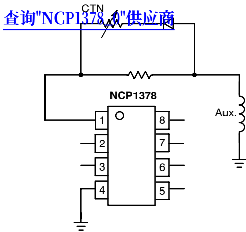
Figure 24. A simple CTN triggers the latchoff as soon as the temperature exceeds a given setpoint.
