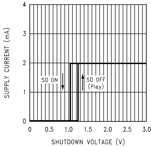
Shutdown Hysteresis Voltage
