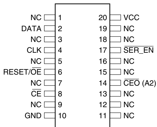
20-lead SOIC (1)
