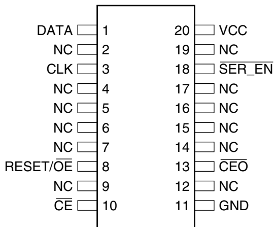
20-lead SOIC (1)
