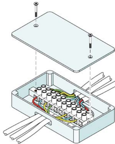
Junction Box
