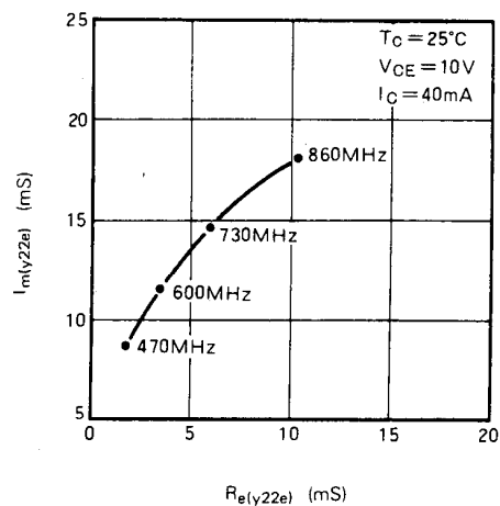
OUTPUT ADMITANCE VS. FREQUENCY
