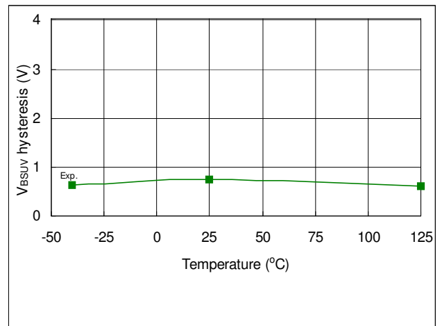
Fig. 29. V_{BS} Supply UV Hysteresis vs. Temperature
