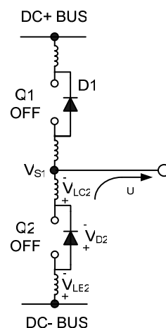
Figure 19: V_S negative
