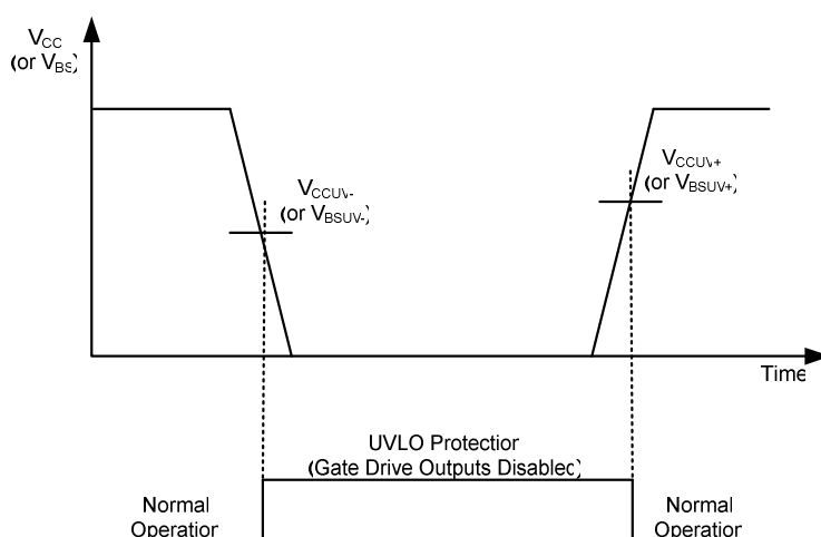
Figure 9: UVLO protection
