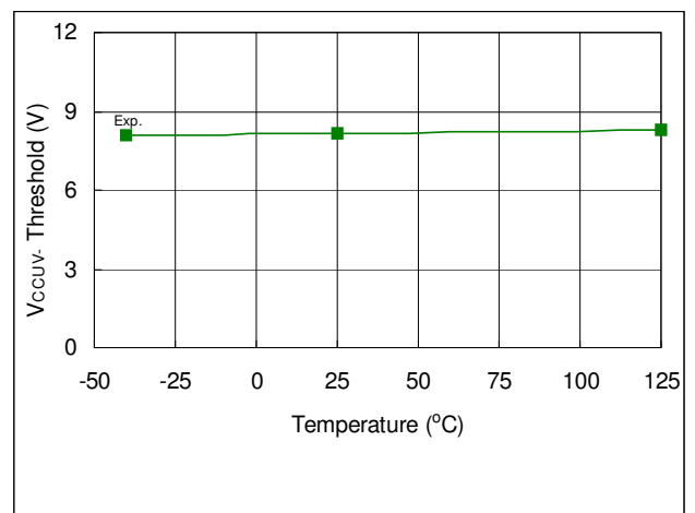
Fig. 33. V_{CCUV-} Threshold vs. Temperature
