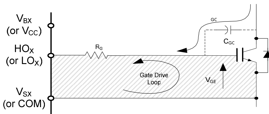
Figure 21: Antenna Loops
