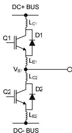
Figure 17: Parasitic Elements
