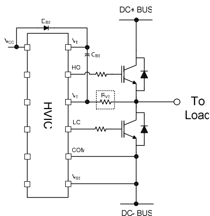
Figure 22: V_S resistor
