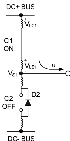
Figure 18: V_S positive
