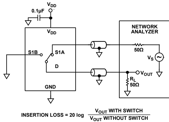
Figure 28. Bandwidth
