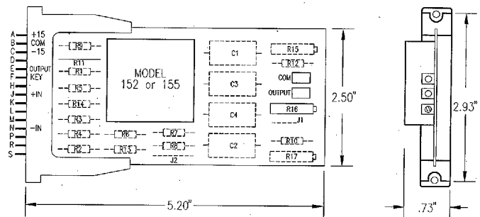
FIGURE 6. MK150 Mounting Kit Dimensions
