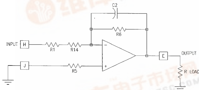
FIGURE 1. Inverting Amplifier
