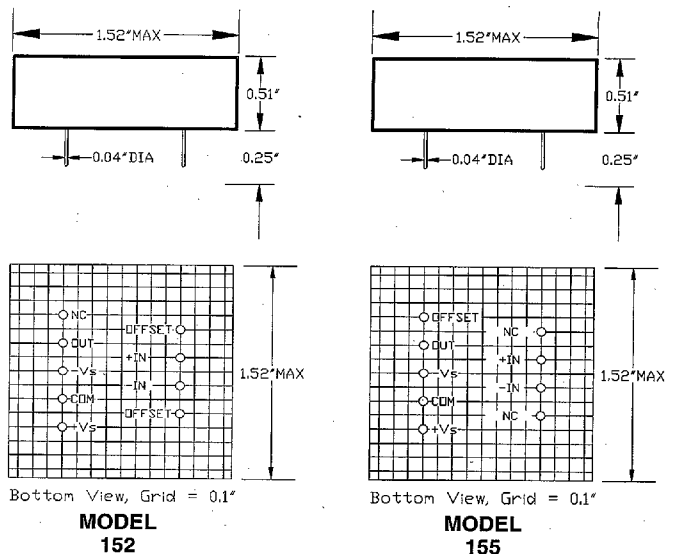
FIGURE 7. Outline Dimensions
