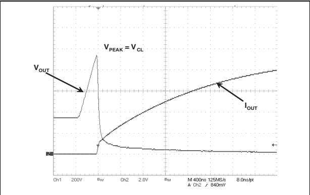
Figure 19. Typical current and voltage waveforms across the ACST12 during IEC 61000-4-5 standard test
