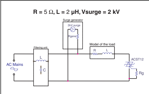
Figure 18. Overvoltage ruggedness test circuit for resistive and inductive loads for IEC 61000-4-5 standards
