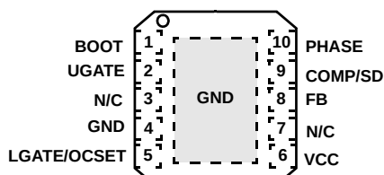
ISL6545 (10 LD 3x3 DFN) TOP VIEW
