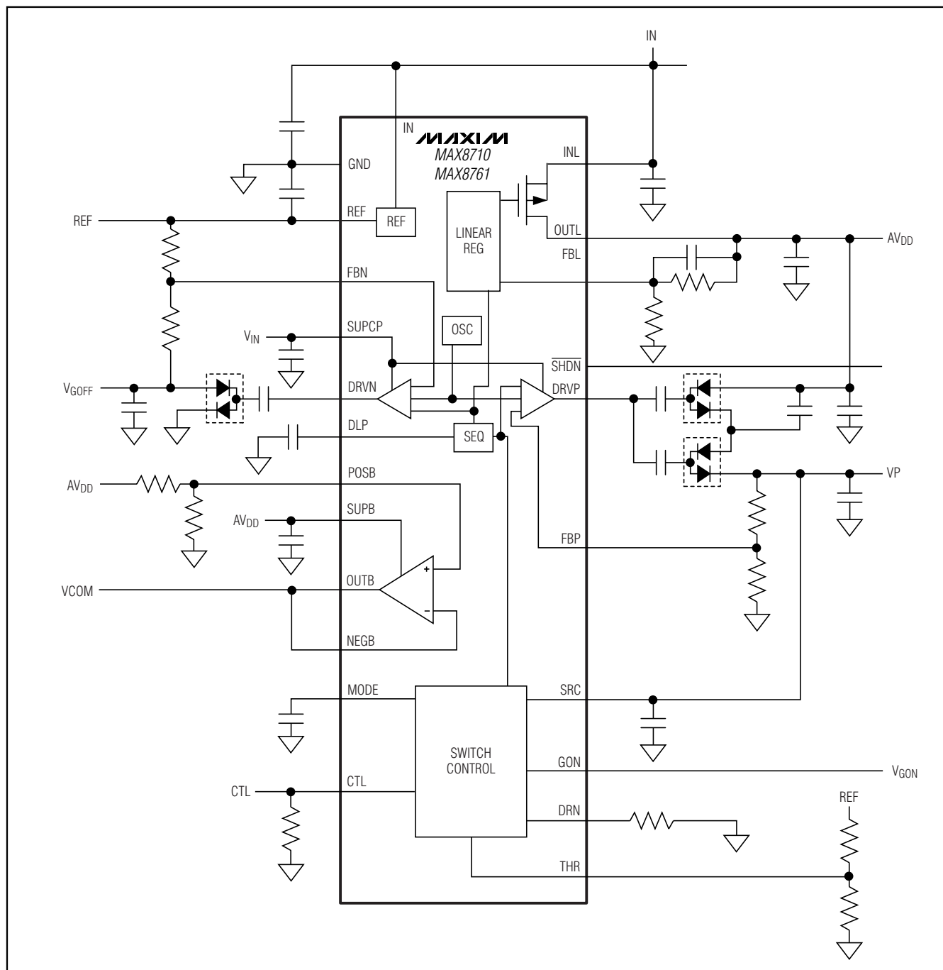
Figure 4. MAX8710/MAX8761 Functional Diagram
