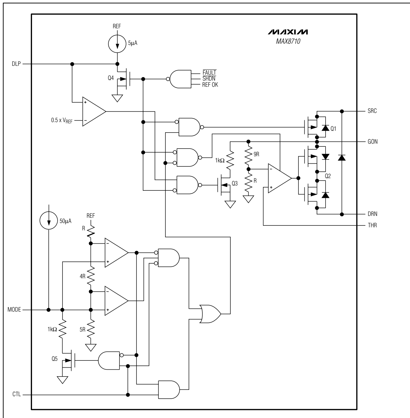
Figure 6. MAX8710 High-Voltage Switch Control
