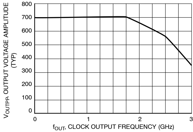
Figure 4. Output Voltage Amplitude (V OUTPP ) versus Clock Output Frequency at Ambient Temperature (Typical)
