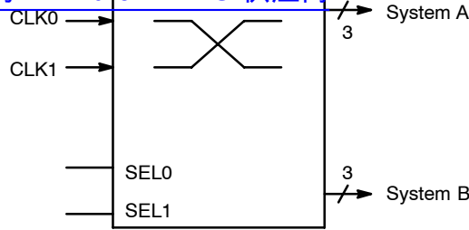
Figure 6. 2 x 2 Clock Switch
