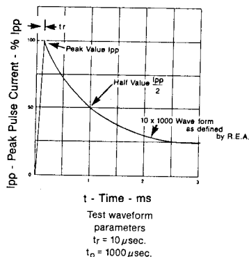
FIGURE 3 PULSE WAVEFORM
