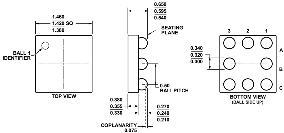
Figure 55. 8-Ball Wafer Level Chip Scale Package [WLCSP] (CB-8-2) Dimensions shown in millimeters
