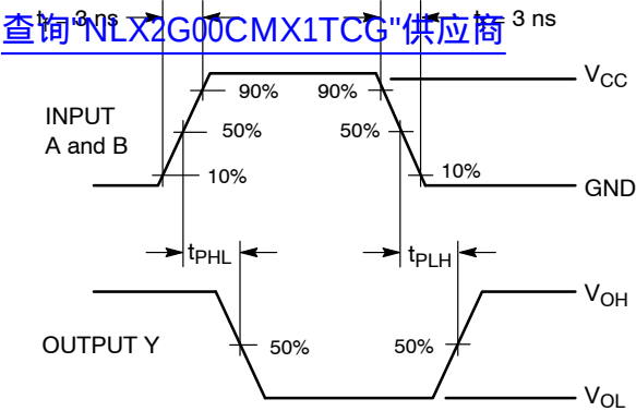
Figure 3. Switching Waveform
