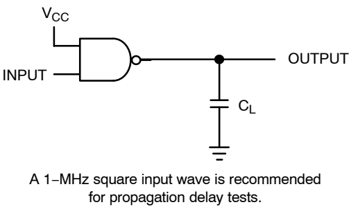
Figure 4. Test Circuit
