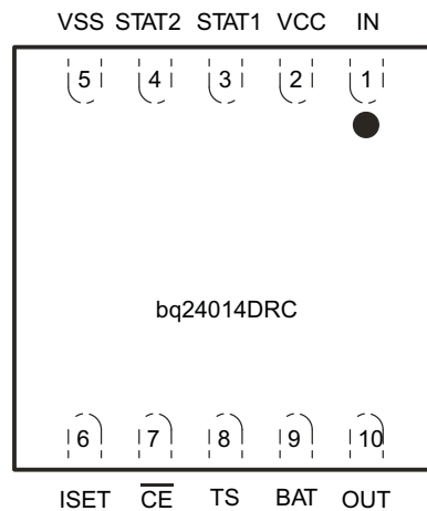
DRC PACKAGE (TOP VIEW)
