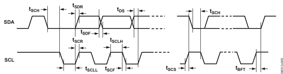
Figure 5. I²C Port Timing
