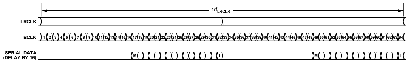
Figure 67. Serial Audio Data Delay by 16 Example
