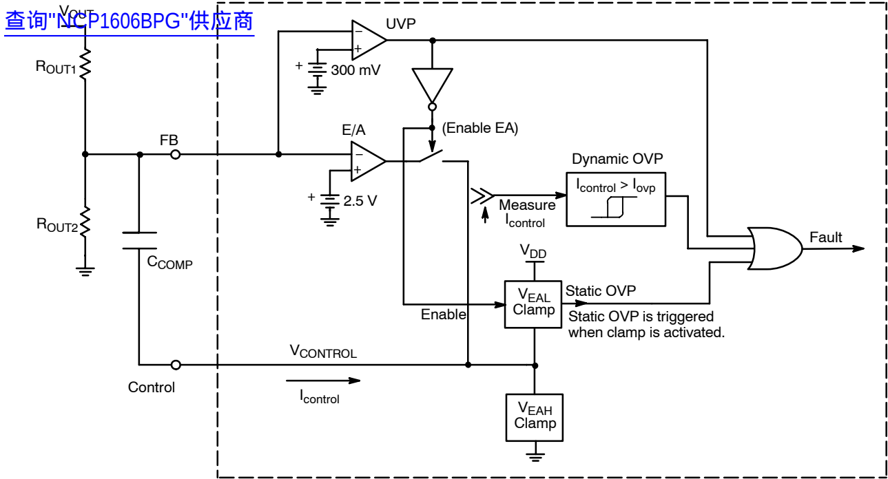
Figure 34. OVP and UVP Circuit Blocks
