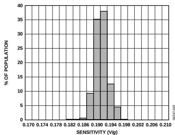
Figure 20. Y-Axis Sensitivity at 25°C, V_S = 2\text{ V}
