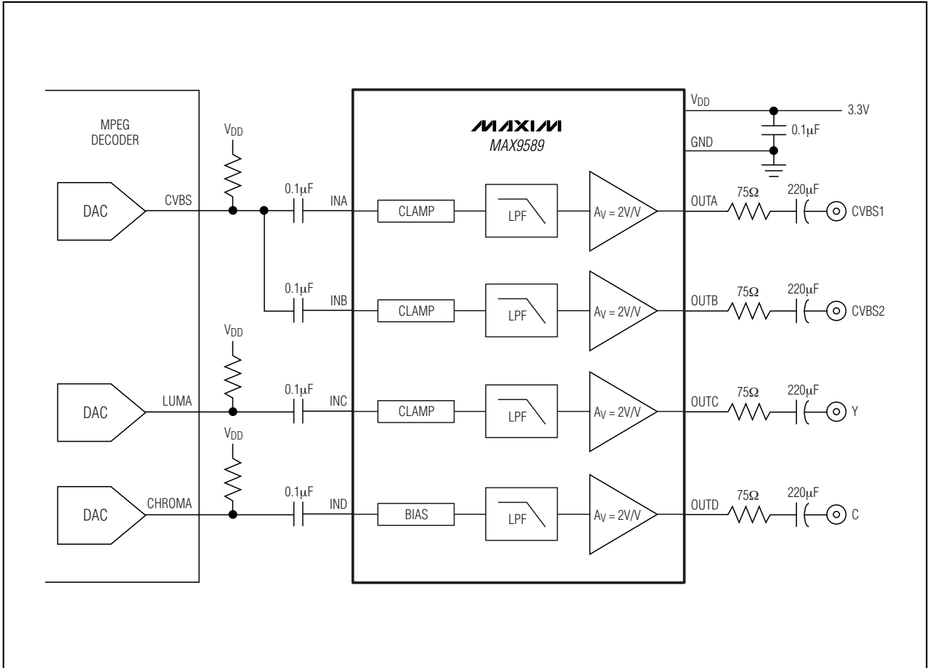
Figure 3. AC-Coupled Outputs
