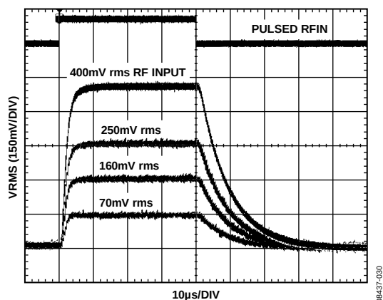
Figure 30. Output Response to Various RF Input Pulse Levels, 3.0 V Supply, 900 MHz Frequency, C_{FLTR} = Open, C_{OUT} = 10 nF, R_{OUT} = 1 k \Omega
