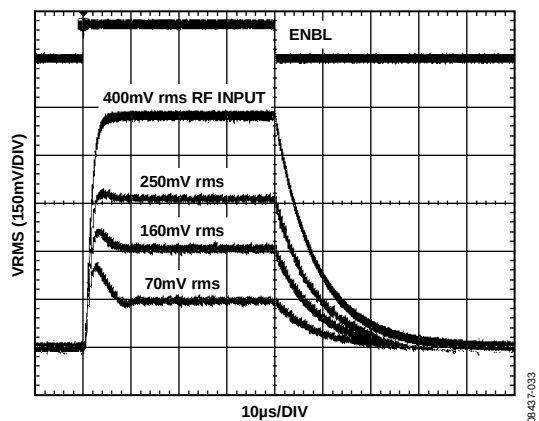
Figure 33. Output Response to Enable Gating at Various RF Input Levels, 3.0 V Supply, 900 MHz Frequency, C_{FLTR} = Open, C_{OUT} = 10 nF, R_{OUT} = 1 k \Omega
