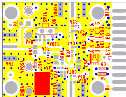
Figure 48. Layout of Evaluation Board, Component Side
