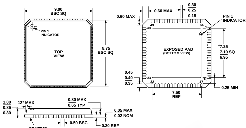
Figure 61. 64-Lead Lead Frame Chip Scale Package [LFCSP_VQ]
