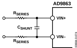
Figure 47. Typical Input
