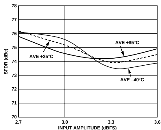
Figure 21. AD9863 Rx Path Single-Tone SFDR Performance vs. ADC_AVDD and Temperature
