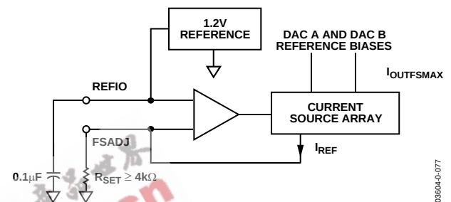
Figure 51. Reference Circuitry
