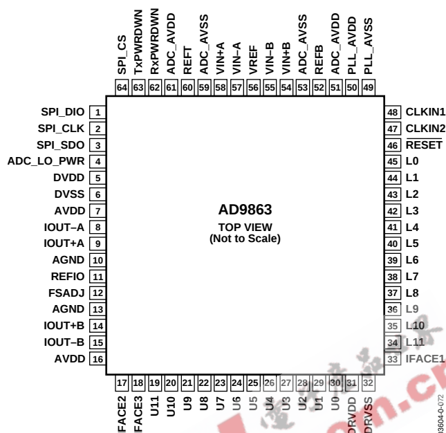
Figure 3. Pin Configuration
