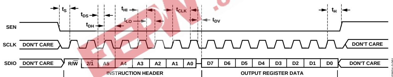
Figure 56. 1-Byte Serial Register Readback in MSB First Mode, SDIO BiDir Bit Set Logic High (Default, 3-Wire Mode)
