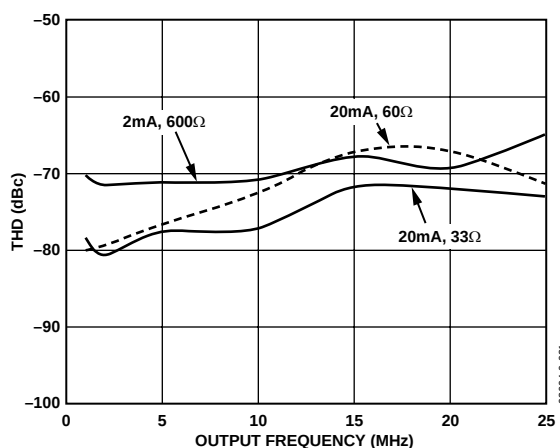
Figure 24. AD9863 Tx Path THD vs. Output Frequency of Tx Channel A
