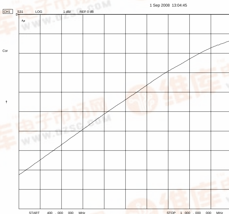
Frequency Response (1 dB/div)
