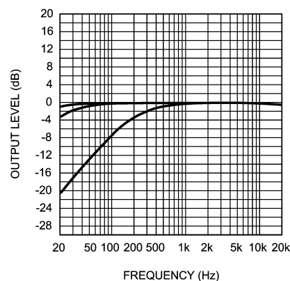
Frequency Response vs Input Capacitor Size R_L = 8\Omega
