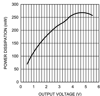
Power Dissipation vs Output Power V_{DD} = 3.3V , R_L = 2\mu F + 30\Omega , f = 1kHz
