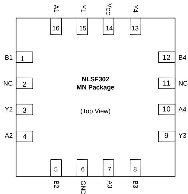
Figure 2. PIN ASSIGNMENT (QFN-16)
