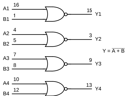
Figure 1. LOGIC DIAGRAM
