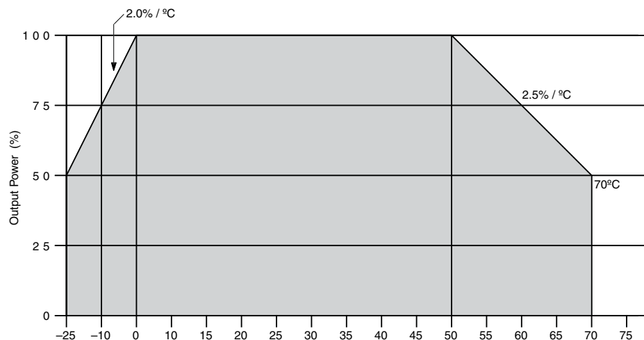
Figure 3. Temperature Derating
