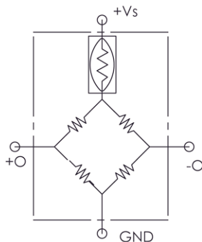
EQUIVALENT CIRCUIT
