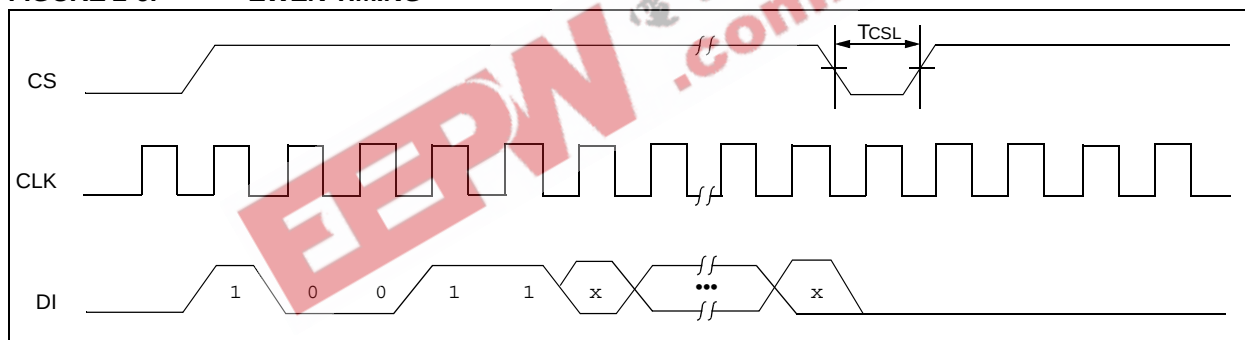
FIGURE 2-6: EWEN TIMING
