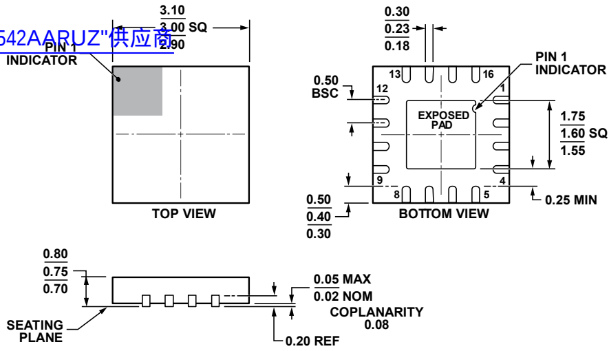
Figure 43. 16-Lead Lead Frame Chip Scale Package [LFCSP] (CP-16-22)
