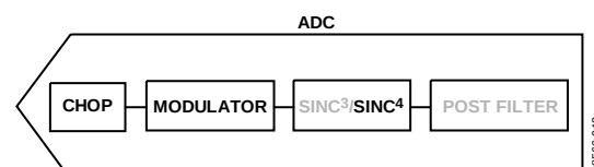
Figure 43. Chop Enabled
