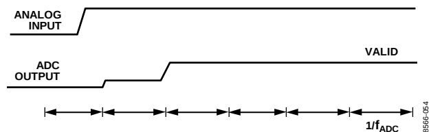
Figure 55. Step Change on Analog Input, \text{Sinc}^4 Filter
