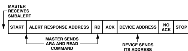
Figure 6. Use of \overline{\text{SMBALERT}}
