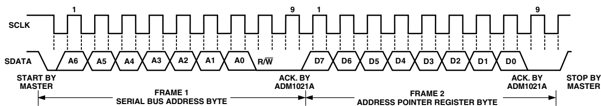
Figure 4. Writing to the Address Pointer Register Only
