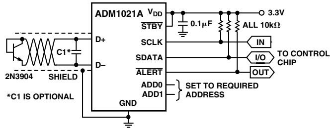
Figure 8. Typical Application Circuit
