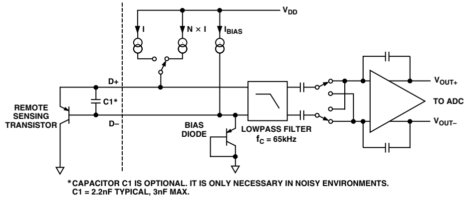
Figure 2. Input Signal Conditioning
