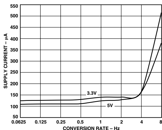
TPC 8. Operating Supply Current vs. Conversion Rate
