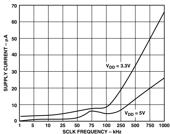
TPC 6. Standby Supply Current vs. Clock Frequency
