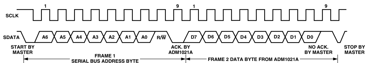
Figure 5. Reading Data from a Previously Selected Register
