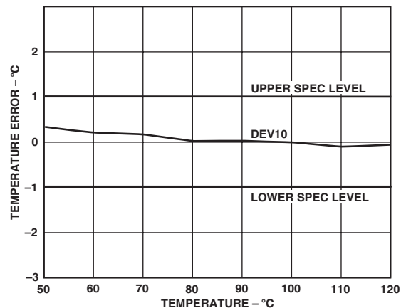
TPC 4. Temperature Error of ADM1021A vs. Pentium III Temperature
