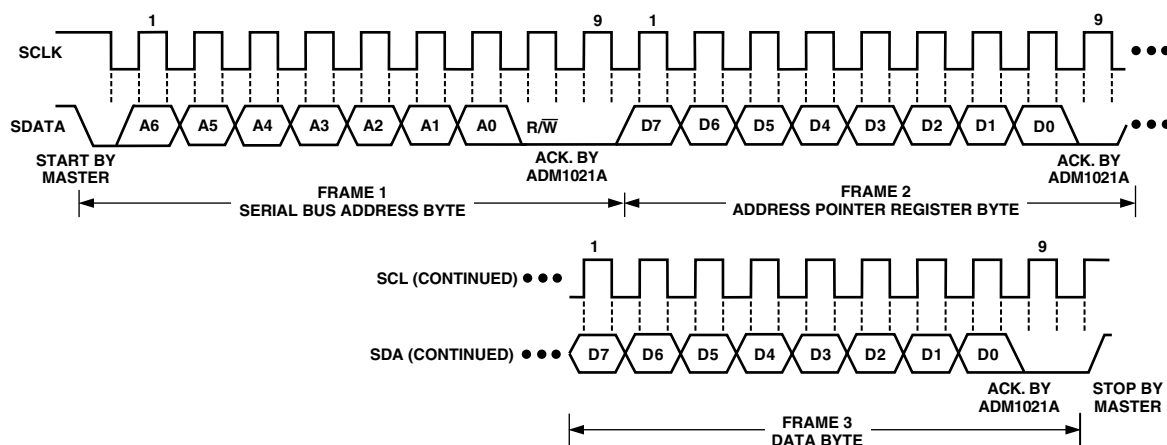
Figure 3. Writing a Register Address to the Address Pointer Register, then Writing Data to the Selected Register
