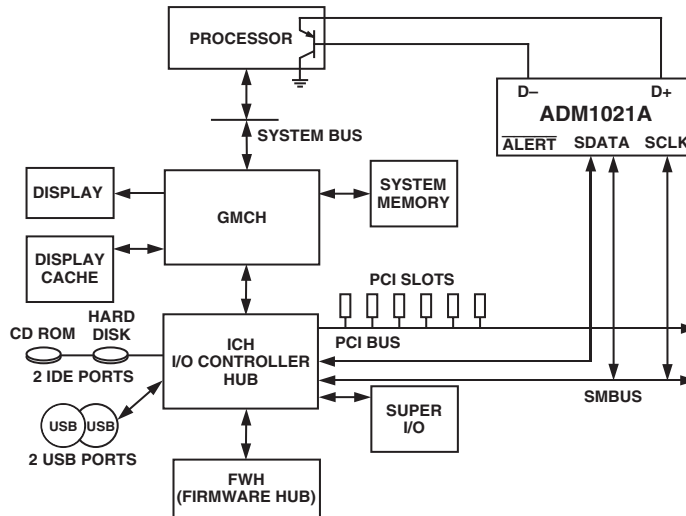
Figure 9. Typical System Using ADM1021A
