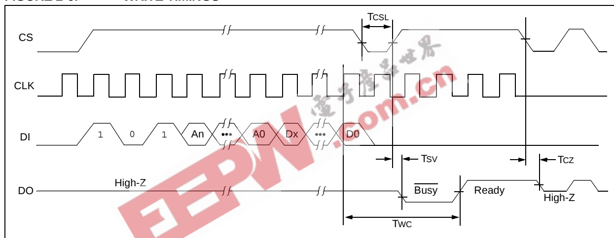
FIGURE 2-6: WRITE TIMINGS
