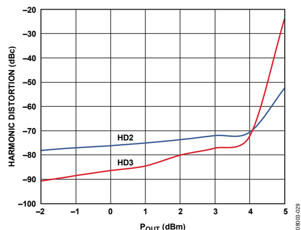
Figure 19. Harmonic Distortion (HD2/HD3) vs. Power ( P_{OUT} ), Frequency 140 MHz, A_v = 15.5 dB
