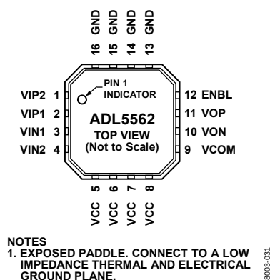
Figure 2. Pin Configuration
